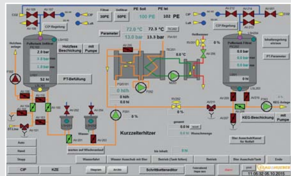
Touch Panel
